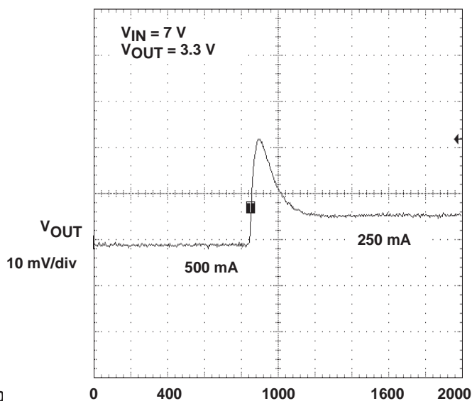
Figure 17. Load Step 500 mA Transition to 250 mA (Circuit Shown in Figure 9.)
