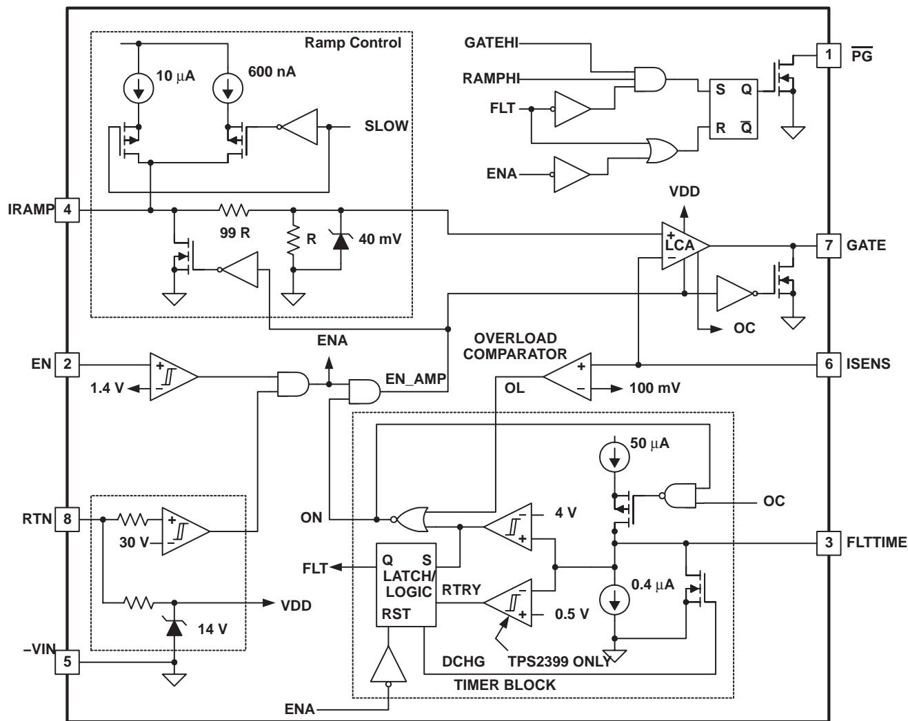
Figure 19. Block Diagram
