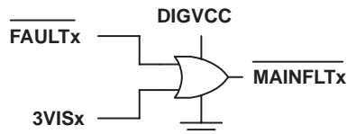
Figure 11. \overline{\text{MAINFLT}} Output Signal
