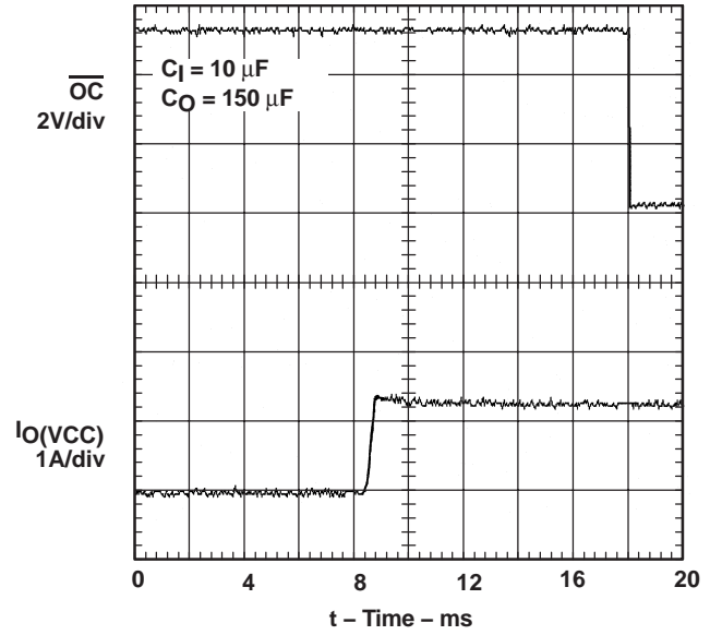
Figure 6. OC Response With 3.3VIN-to-xVCC Switch Output Turned on Into a Short
