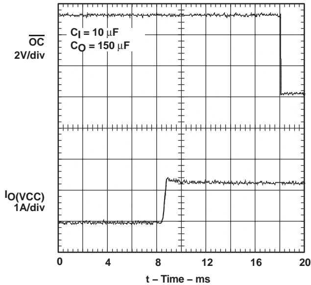
Figure 5. OC Response With 5VIN-to-xVCC Switch Output Turned on Into a Short
