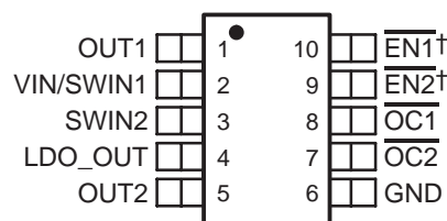
TPS2147, TPS2157 MSOP (DGQ) PACKAGE (TOP VIEW)
