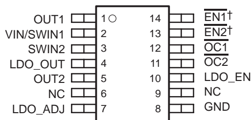
TPS2145, TPS2155 TSSOP (PWP) PACKAGE (TOP VIEW)
