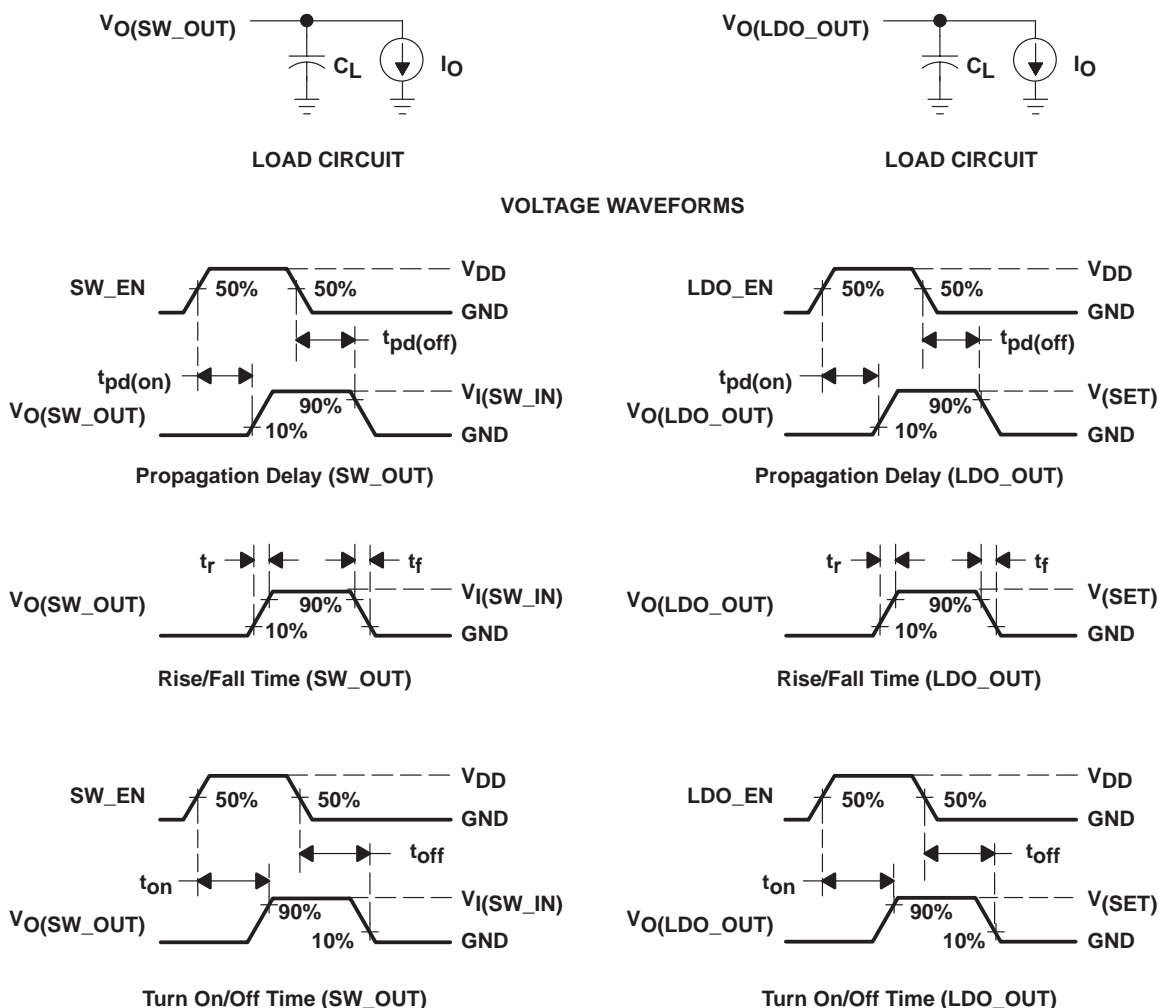
Figure 1. Test Circuits and Voltage Waveforms
