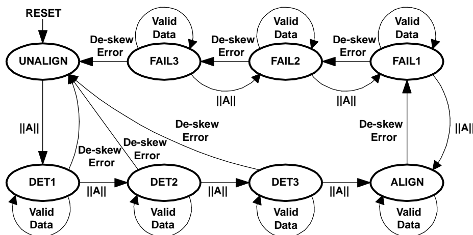
Figure 12. Column De-Skew State Machine
