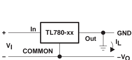
Figure 2. Positive Regulator in Negative Configuration ( V_I Must Float)
