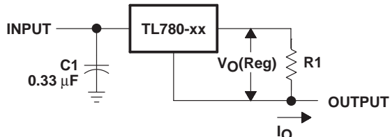
Figure 3. Current Regulator
