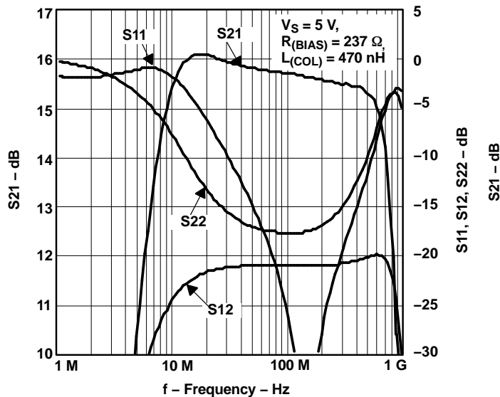
Figure 19. S-Parameters of THS9000 mounted on the standard EVM with V_S = 5\text{ V} , R_{(BIAS)} = 237\Omega , and L_{(COL)} = 470\text{ nH}
