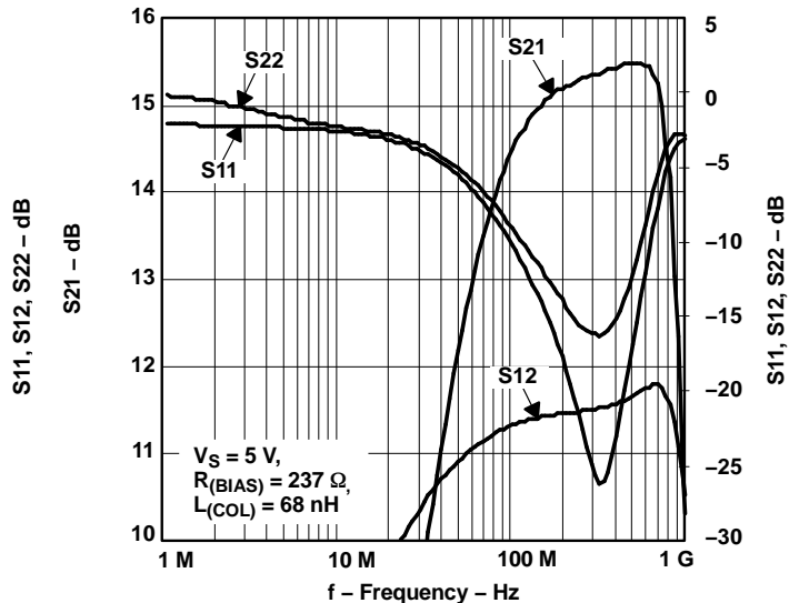
Figure 20. S-Parameters of THS9000 mounted on the standard EVM with V_S = 5\text{ V} , R_{(BIAS)} = 237\Omega , and L_{(COL)} = 68\text{ nH}
