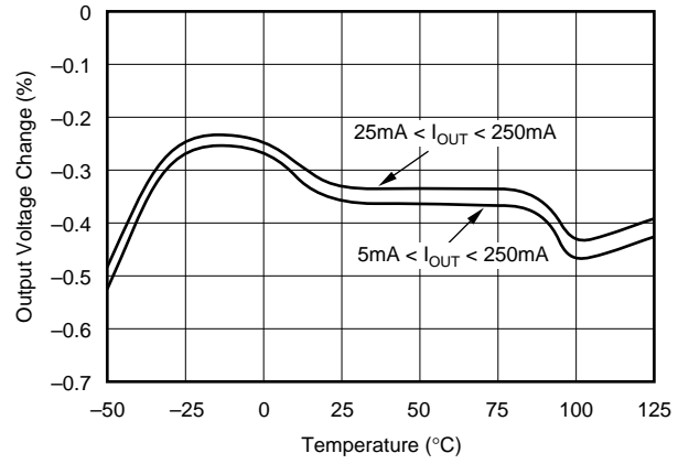
LOAD REGULATION vs TEMPERATURE (V_{\text{IN}} = V_{\text{OUT}} + 1\text{V})
