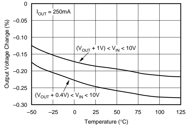
LINE REGULATION vs TEMPERATURE
