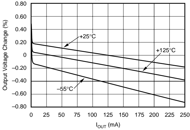
OUTPUT VOLTAGE CHANGE vs I_{\text{OUT}} (V_{\text{IN}} = V_{\text{OUT}} + 1\text{V}, \text{Output Voltage \% Change} Referred to I_{\text{OUT}} = 125\text{mA} at +25^\circ\text{C} )
