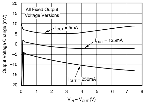
LINE REGULATION (Referred to V_{\text{IN}} = V_{\text{OUT}} + 1\text{V} at I_{\text{OUT}} = 125\text{mA} )
