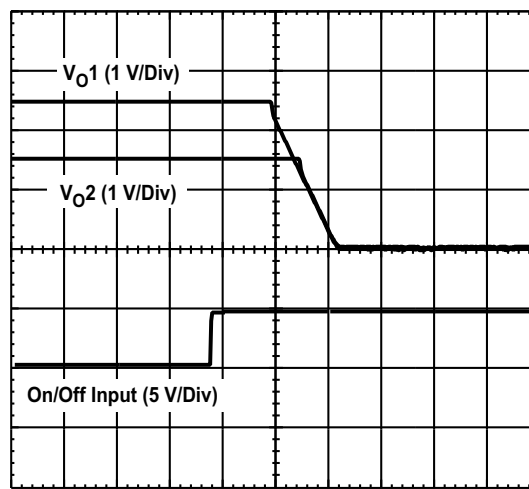
Figure 13. Simultaneous Power Down With Auto-Track Control
