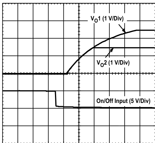
Figure 12. Simultaneous Power Up With Auto-Track Control
