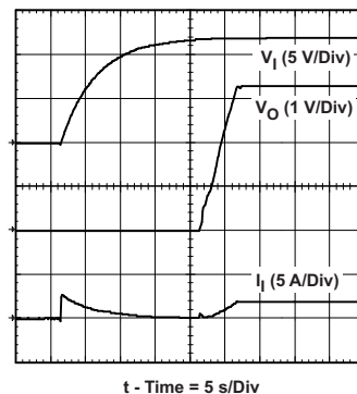
Figure 11. Power-Up Waveforms
