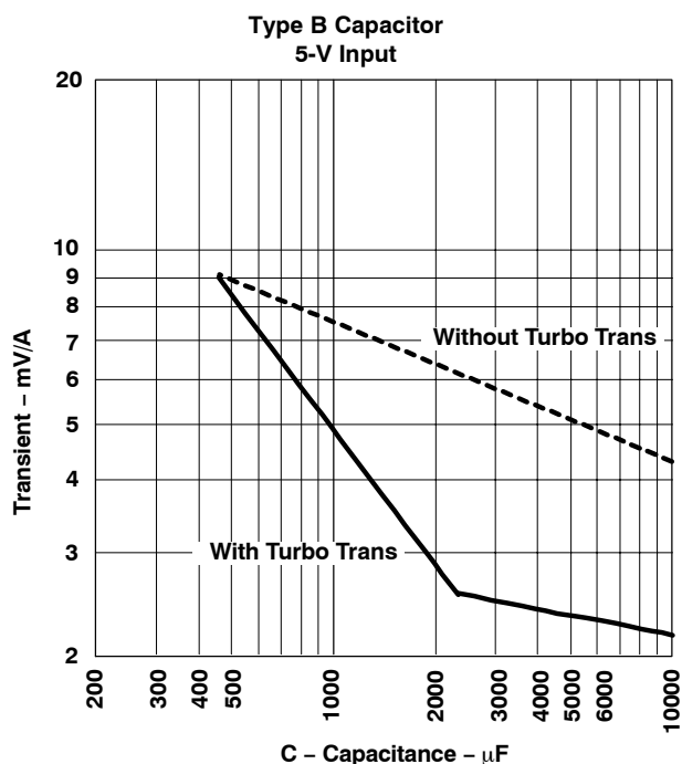
Figure 7. Capacitor Type B, 1000 \leq C (\mu F) \times ESR (m\Omega) \leq 5000 (e.g. Polymer-Tantalum)
