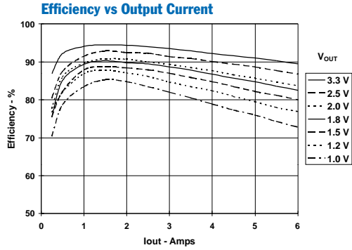
Characteristic Data; V_{in}=5\text{ V} (See Note A)
