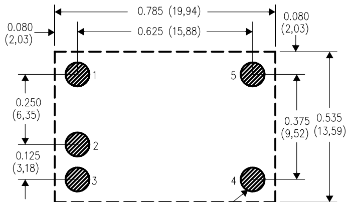
PC LAYOUT
