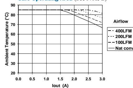
Safe Operating Area (See Note B)
