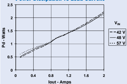
Power Dissipation vs Load Current
