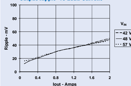
Output Ripple vs Load Current
