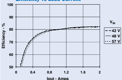
Efficiency vs Load Current
