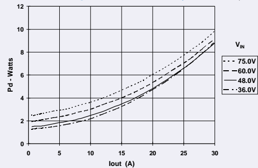
Power Dissipation vs Load Current; V_o = 1.5\text{ V} (See Note A)
