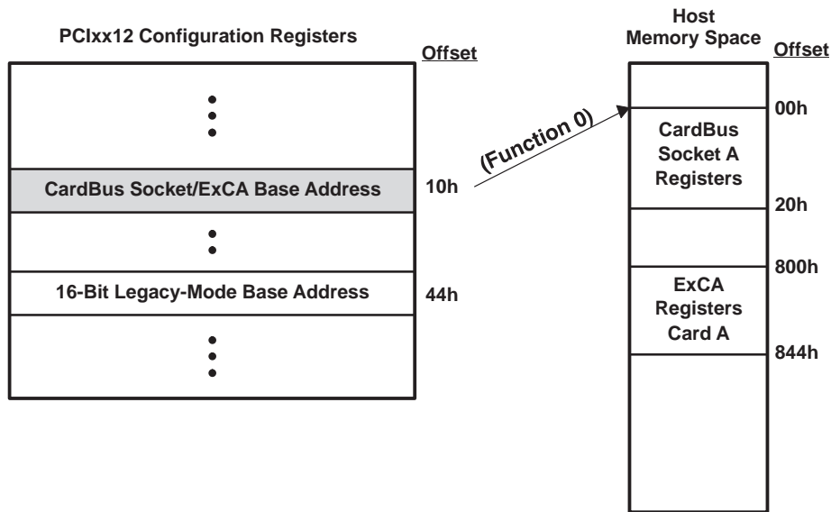
Offsets are from the CardBus socket/ExCA base address register's base address.
