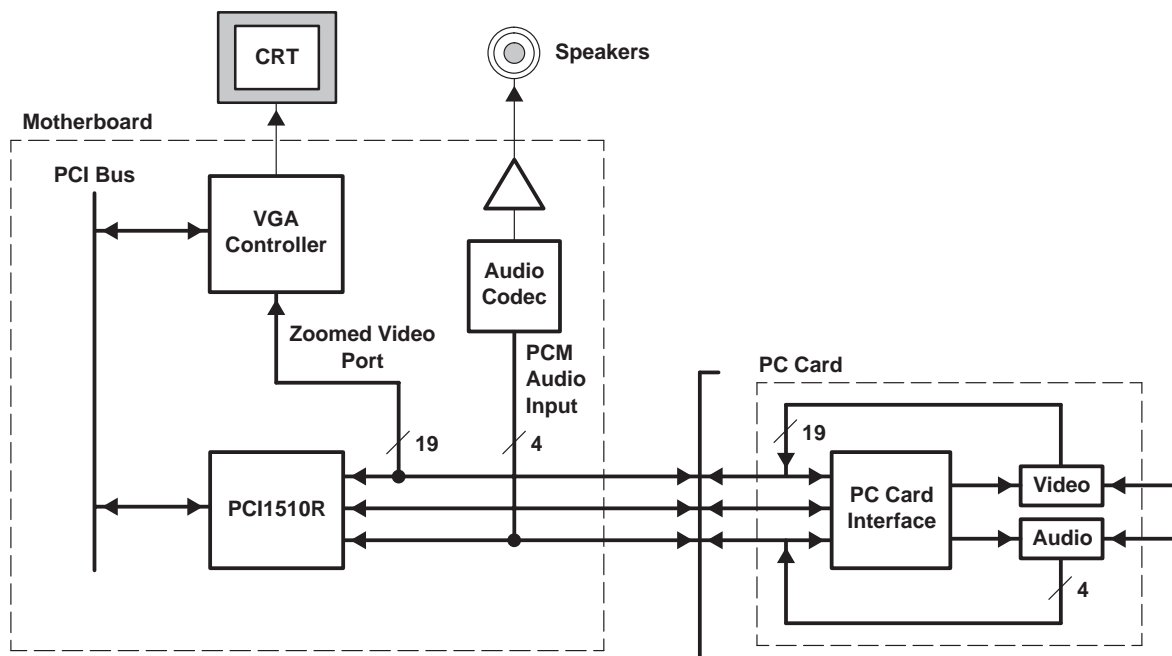
Figure 3-4. Zoomed Video Implementation Using the PCI1510R Controller
