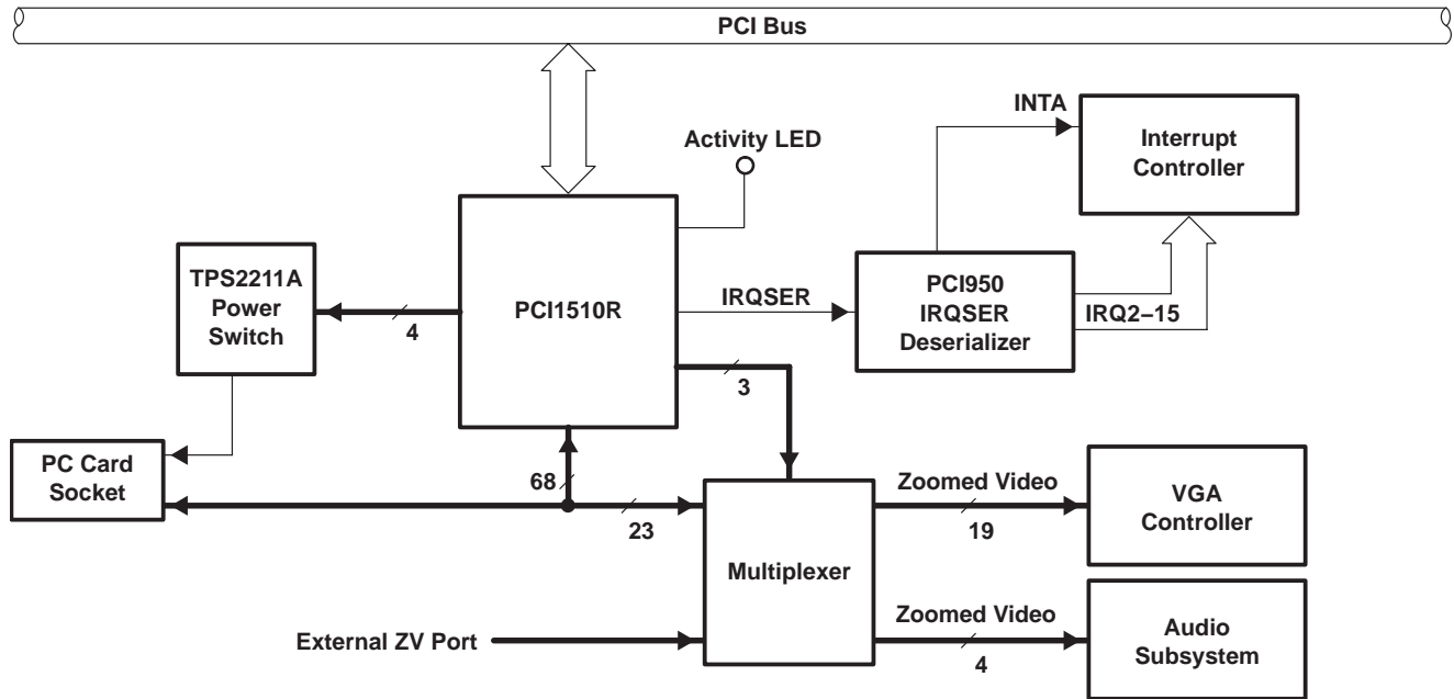
Figure 3–1. PCI1510R Simplified Block Diagram
