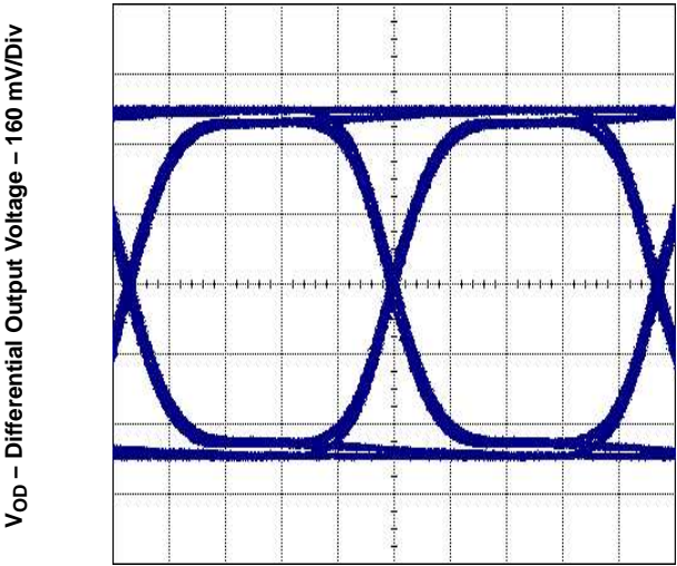
OUTPUT EYE-DIAGRAM AT 4.25 GBPS AND MINIMUM INPUT VOLTAGE (50 mV p-p )
