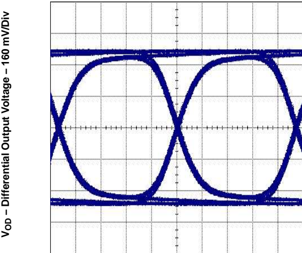
OUTPUT EYE-DIAGRAM AT 4.25 GBPS AND 85°C AND MINIMUM INPUT VOLTAGE (50 mV p-p )
