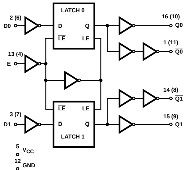
FIGURE 1. LOGIC DIAGRAM
