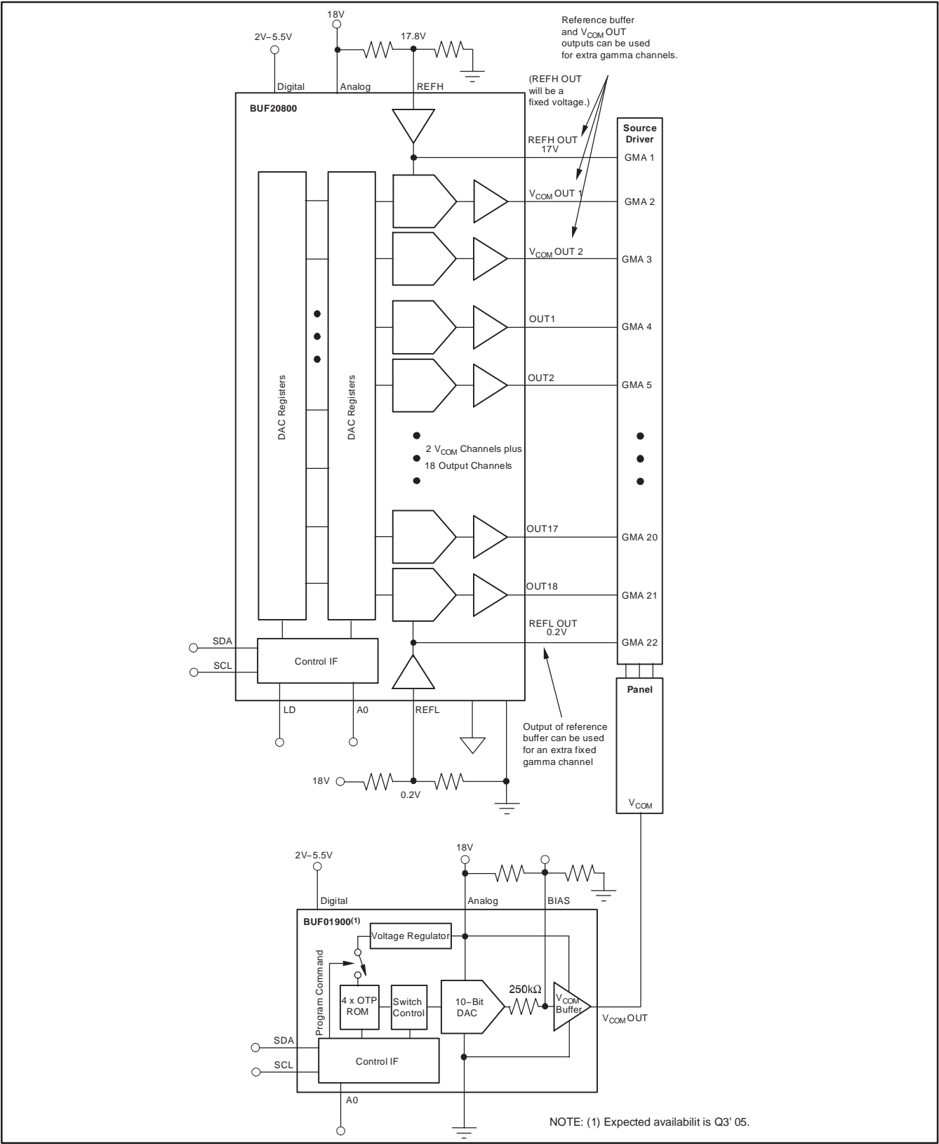
Figure 15. 22-Channel Gamma Solution
