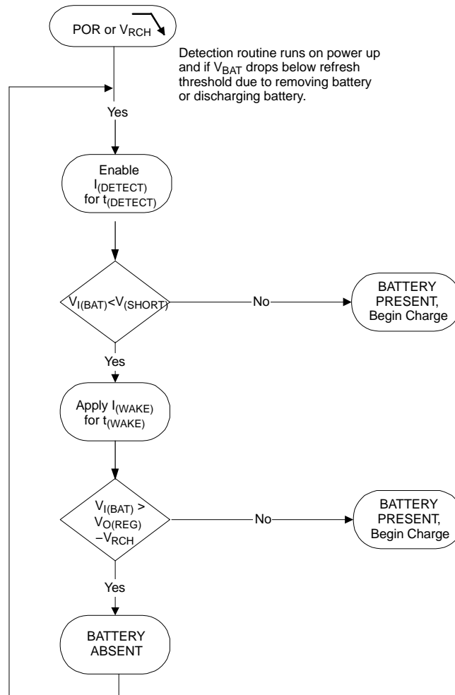
Figure 13. Battery Detection for bq2412x ICs
