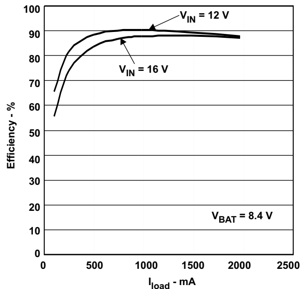
Figure 5. Efficiency 2-Cells
