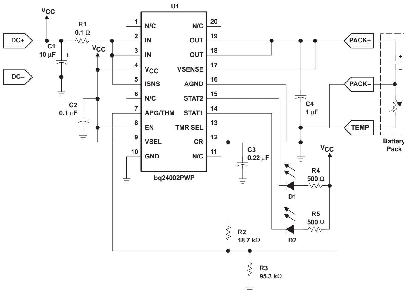
Figure 13. Li-Ion/Li-Pol Charger
