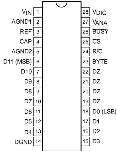
DW PACKAGE (TOP VIEW)
