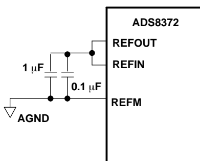
Figure 48. ADS8372 Using Internal Reference
