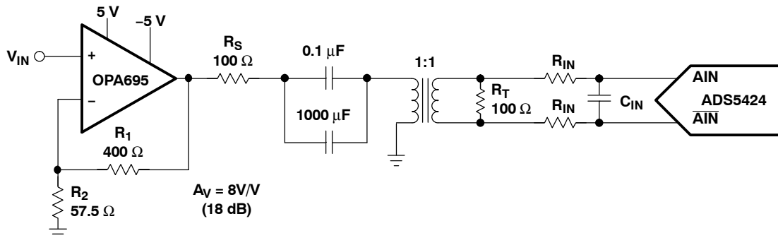
Figure 39. Using the OPA695 With the ADS5424
