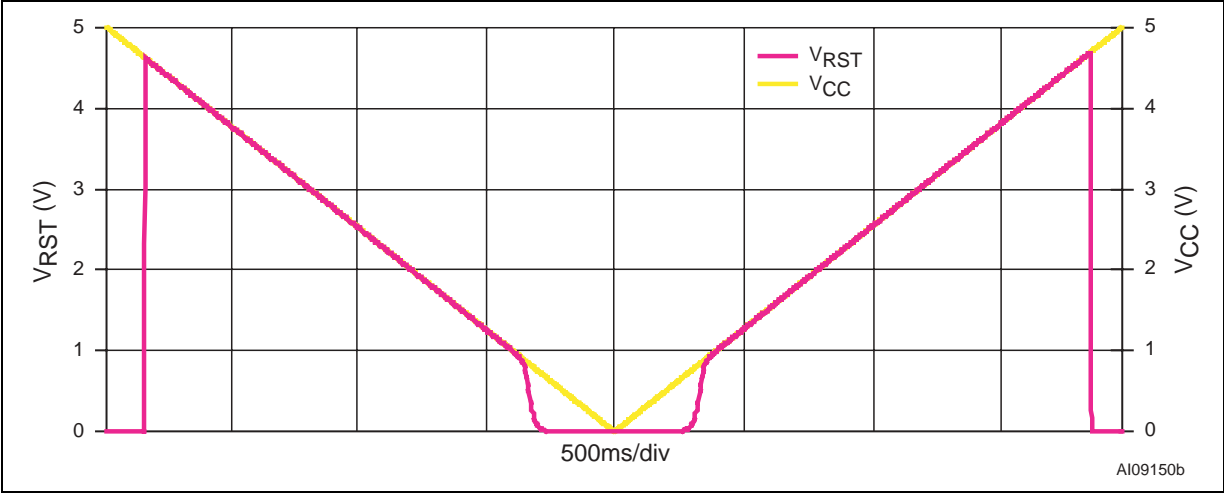
Figure 33. RST Output Voltage vs. Supply Voltage
