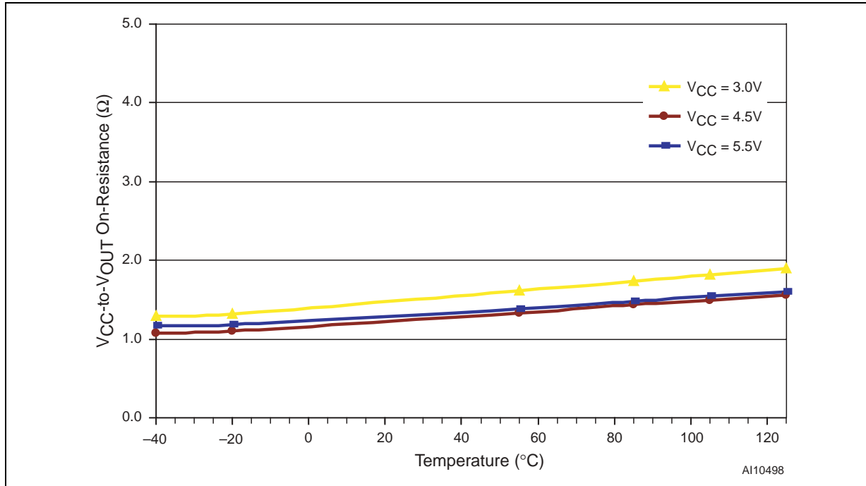
Figure 18. V_{CC} -to- V_{OUT} On-Resistance vs. Temperature
