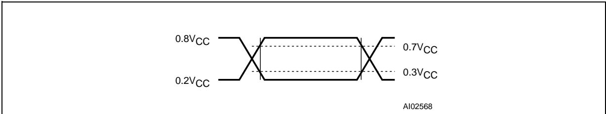
Figure 41. AC Testing Input/Output Waveforms
