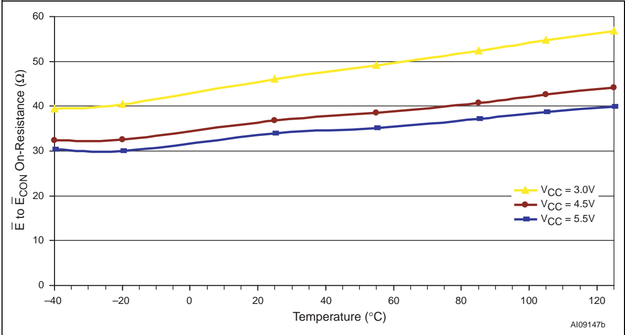
Figure 28. \bar{E} to \bar{E}_{CON} On-Resistance vs. Temperature
