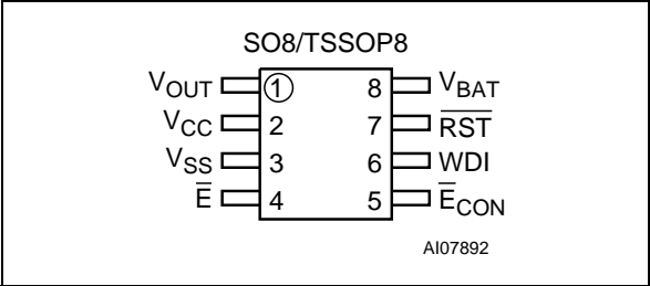
Figure 7. STM818 Connections
