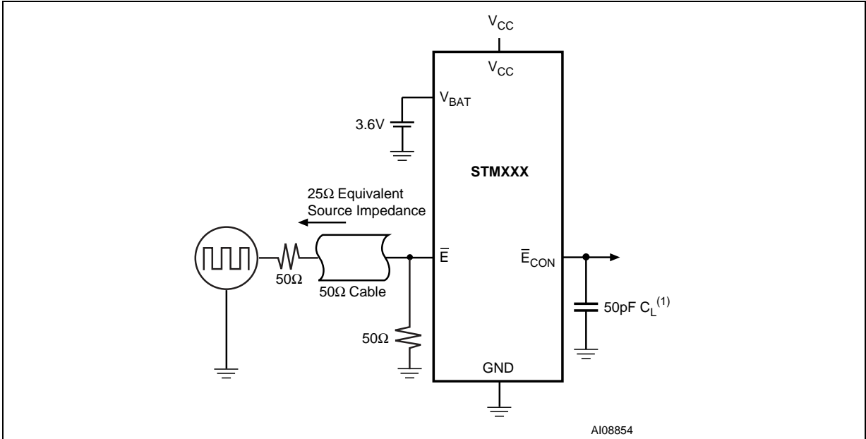
Figure 40. \overline{E} to \overline{ECON} Propagation Delay Test Circuit
