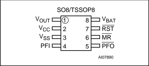
Figure 6. STM703/704/819 Connections
