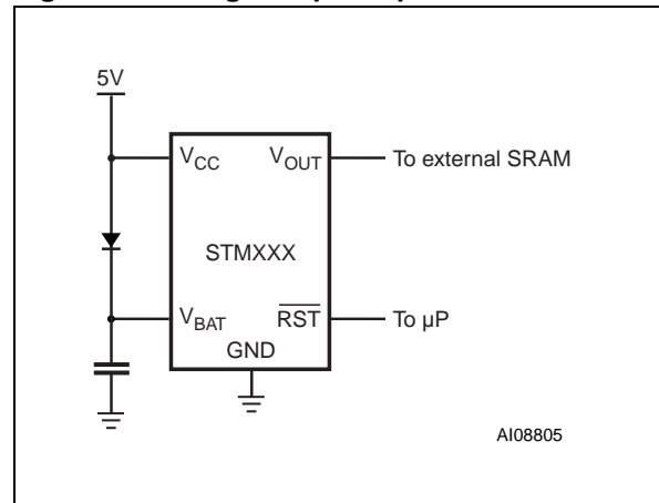
Figure 16. Using a SuperCap™
