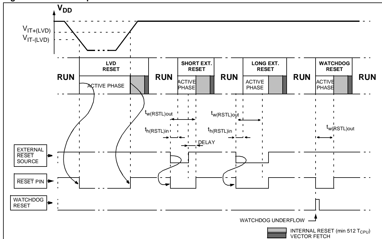
Figure 18. RESET Sequences
