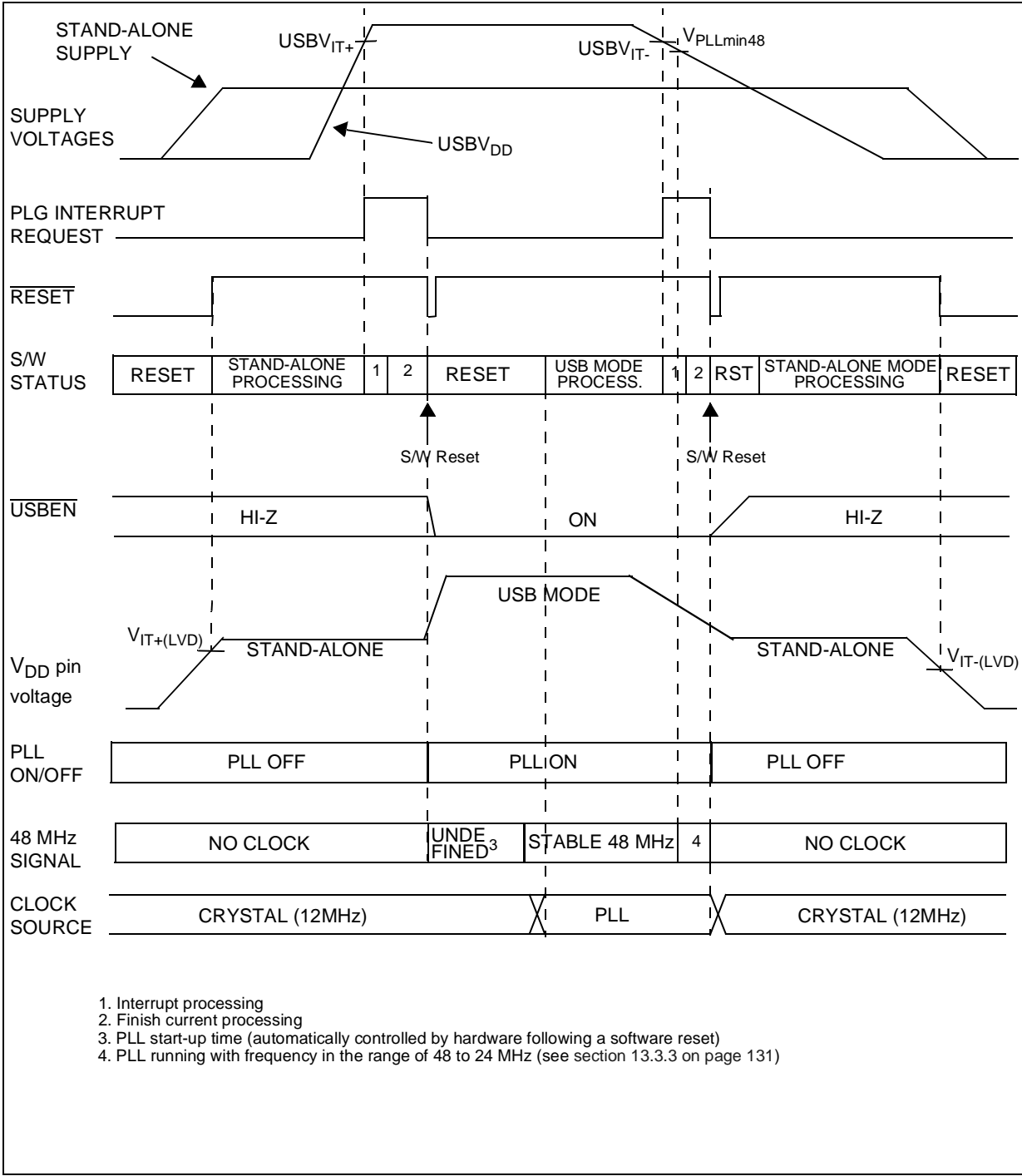
Figure 25. Power Supply Management: Dual Power Supply
