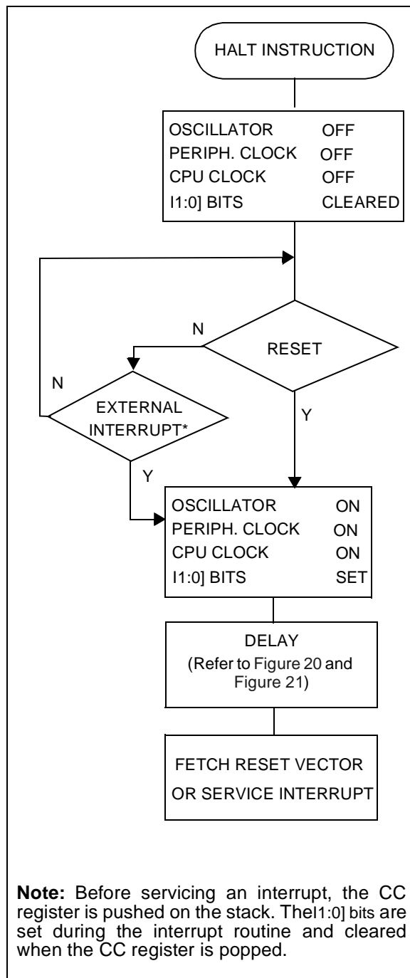
Figure 34. HALT Mode Flow Chart
