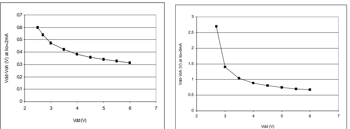
Figure 96. Typical V_{OH} vs. V_{DD}
