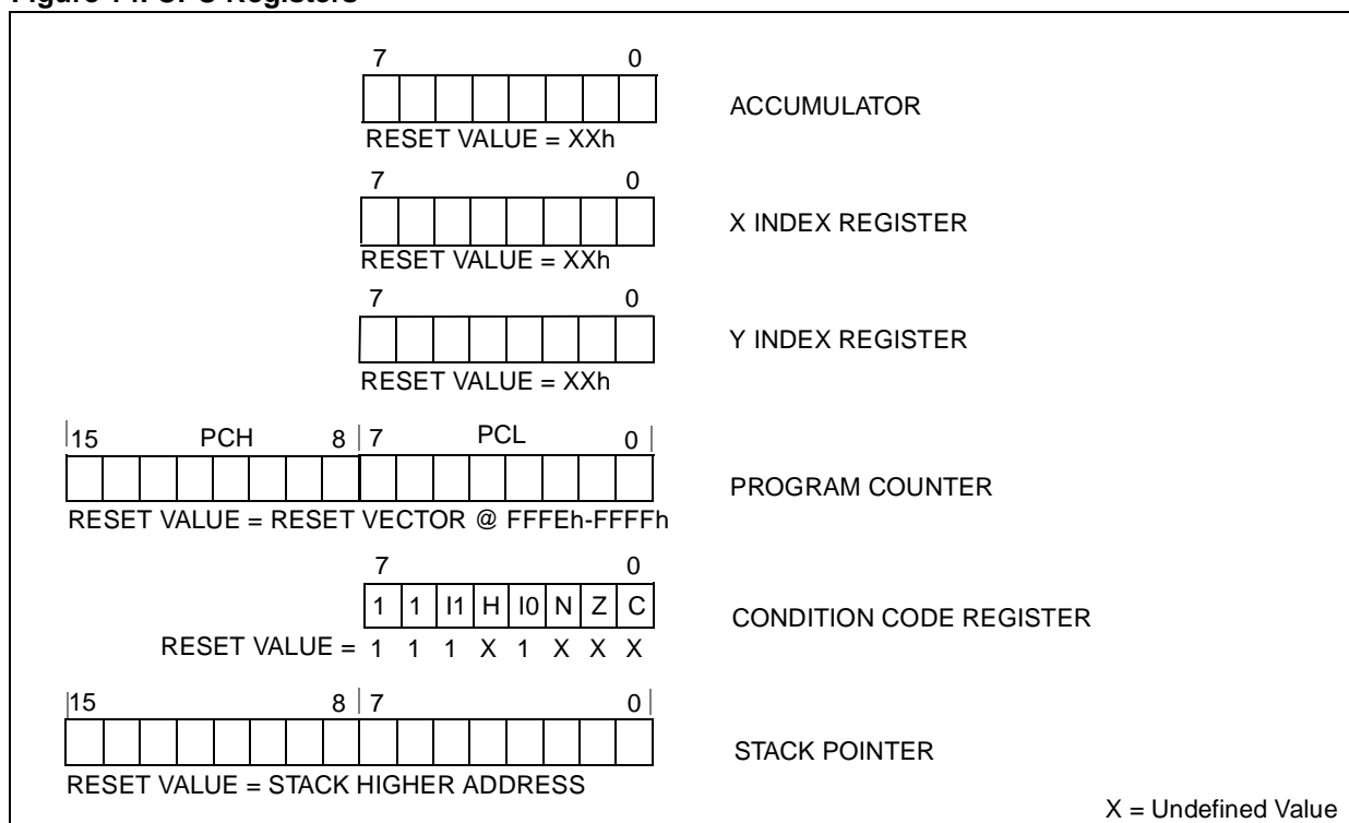
Figure 14. CPU Registers
