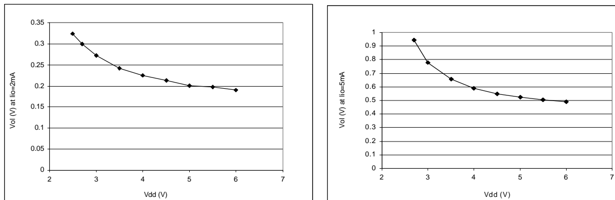
Figure 95. Typical V_{OL} vs. V_{DD} (high-sink I/Os)
