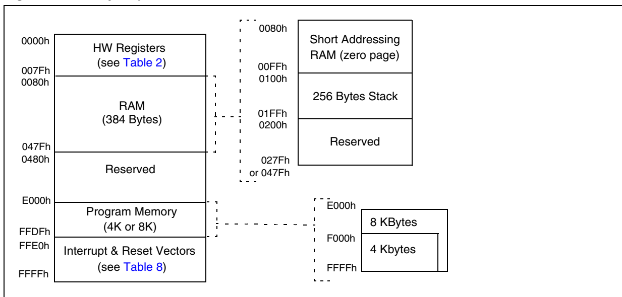
Figure 5. Memory Map
