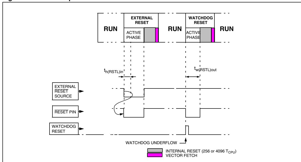
Figure 14. RESET Sequences
