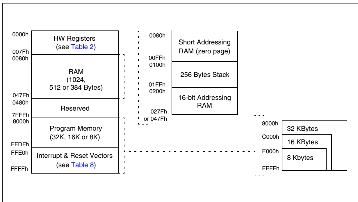
Figure 5. Memory Map
