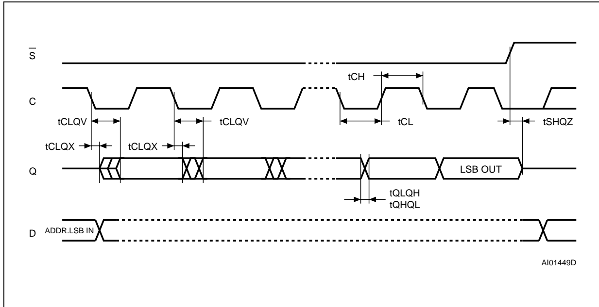
Figure 24. Output Timing
