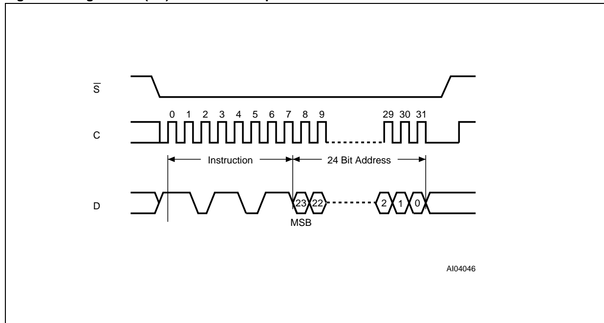
Figure 16. Page Erase (PE) Instruction Sequence
