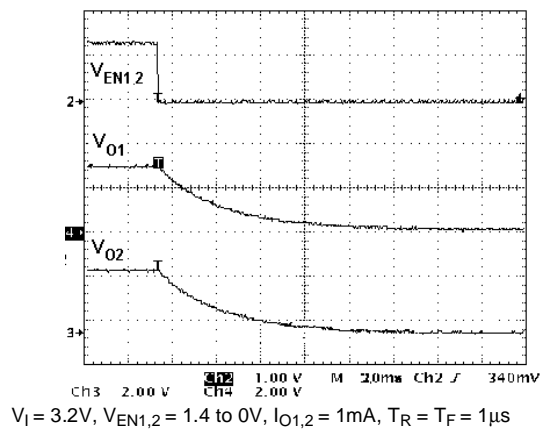
Figure 17: TURN-OFF
