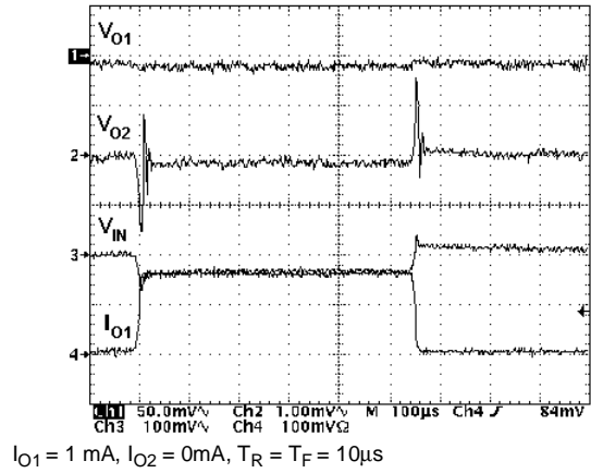
Figure 16: TURN-ON
