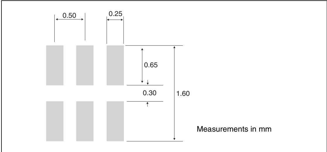
Figure 11. Footprint
