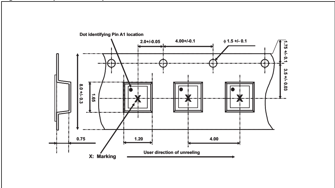
Figure 12. Tape and reel specification
