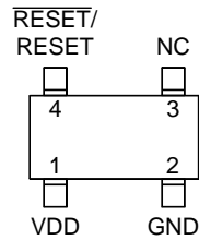
SC-70-4 (R-Type)
