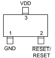
SOT-23-3 (L-Type)
