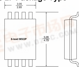
Figure 2. Package Type
