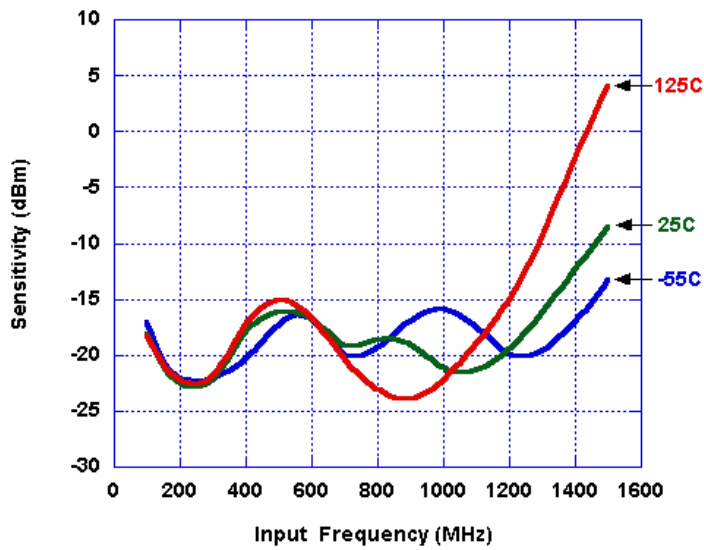
Figure 4. Input Sensitivity
