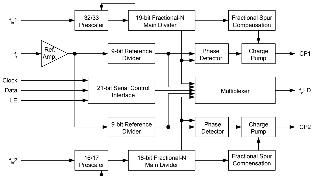
Figure 4. PE3291 Block Diagram
