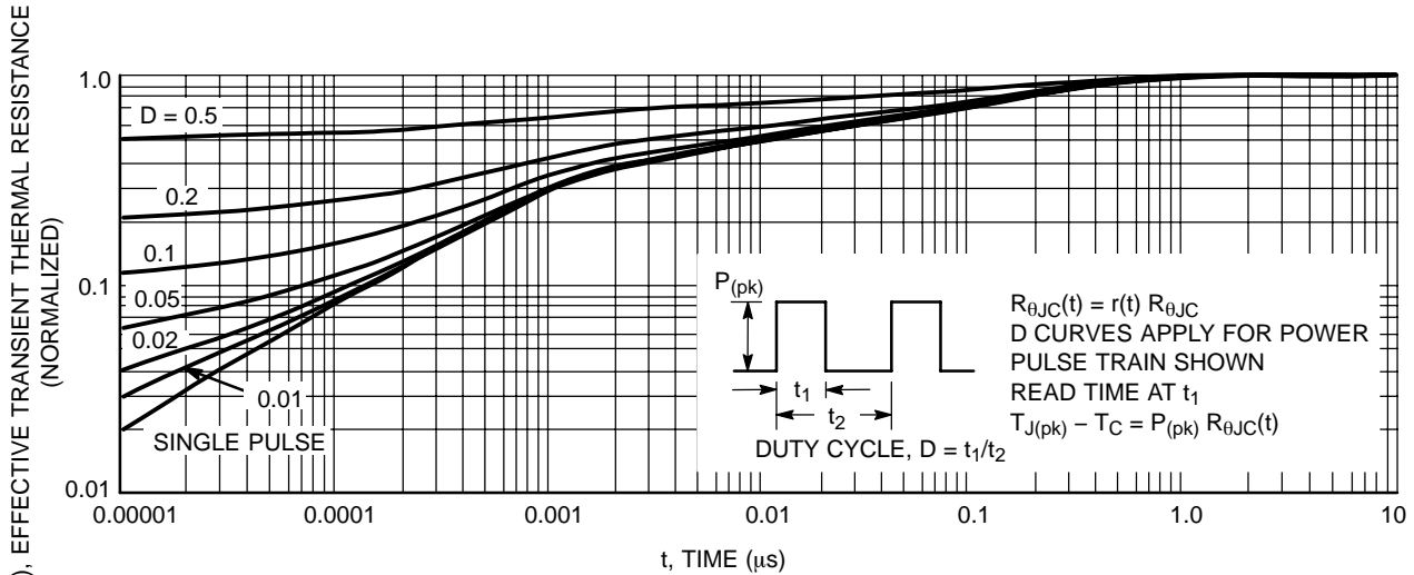
Figure 13. Thermal Response
