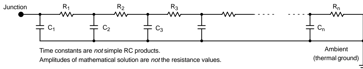
Figure 20. Grounded Capacitor Thermal Network ("Cauer" Ladder)
