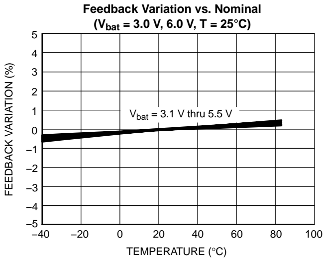
Figure 16. Feedback Voltage Variation
