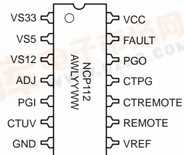
PDIP-14, SOIC-14
