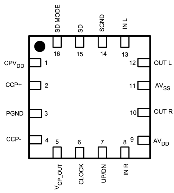
Top View Order Number LM4981SQ See NS Package Number SQA16A
