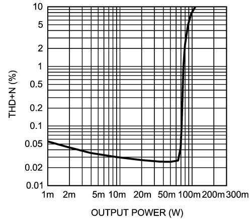
THD+N vs Output Power V_{DD} = 3.6V, R_L = 32\Omega, f = 1kHz, \text{two channels}
