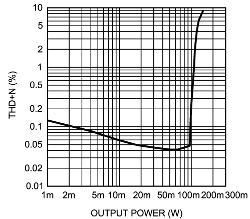
THD+N vs Output Power V_{DD} = 4.2V, R_L = 16\Omega, f = 1kHz, \text{two channels}
