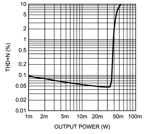
THD+N vs Output Power V_{DD} = 3V, R_L = 32\Omega, f = 1kHz, \text{two channels}
