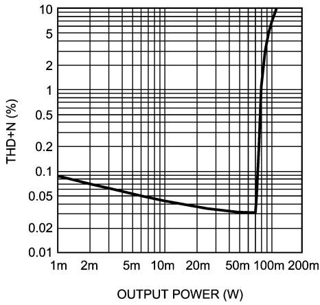
THD+N vs Output Power V_{DD} = 3V, R_L = 32\Omega, f = 1kHz, \text{one channel}
