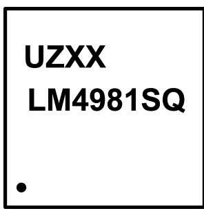
Top View U = Plant Code ZX = Date Code X = Die Traceability Bottom Line = Part Number
