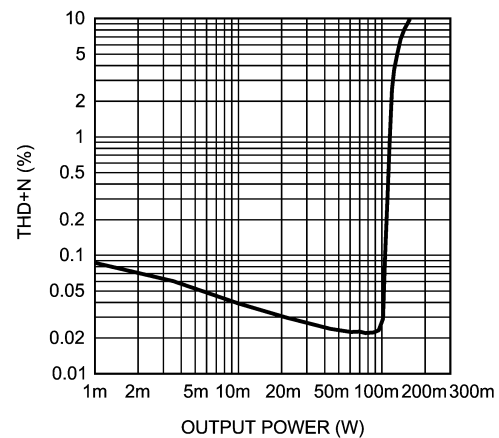
THD+N vs Output Power V_{DD} = 4.2V, R_L = 32\Omega, f = 1kHz, \text{two channels}
