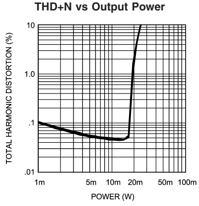
Analog V_{DD} = 2.6V , Digital V_{DD} = 2.6V R_L = 32\Omega , 44.1 kHz Sample Rate R & L Channels Shown, Vol = 3dB, Frequency in = 1kHz
