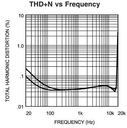
Analog V_{DD} = 5V , Digital V_{DD} = 3V R_L = 32\Omega , Power Level = 50mW R & L Channels Shown, 44.1kHz Sample Rate
