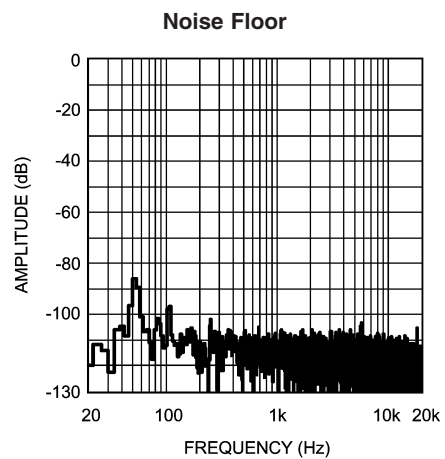
200486E9 Analog V_{DD} = 3V , Digital V_{DD} = 3V R_L = 32\Omega , V_{ol} = 0dB , 44.1kHz Sample Rate
