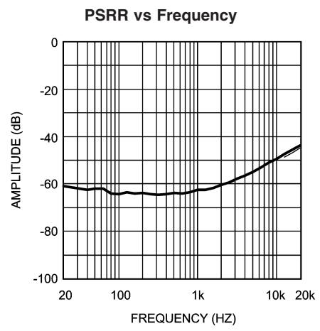
Analog V_{DD} = 5V , Digital V_{DD} = 3V R_L = 32\Omega , Vol = 3dB, 44.1kHz Sample Rate
