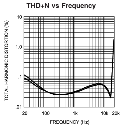
Analog V_{DD} = 3V , Digital V_{DD} = 3V R_L = 32\Omega , Power Level = 12mW R & L Channels Shown, 44.1kHz Sample Rate
