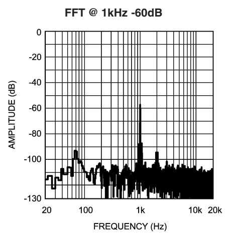
Analog V_{DD} = 3V , Digital V_{DD} = 3V R_L = 32\Omega , Vol = 0dB, 44.1kHz Sample Rate
