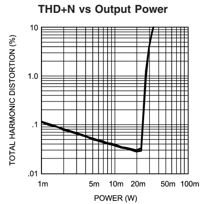
Analog V_{DD} = 3V , Digital V_{DD} = 3V R_L = 32\Omega , 44.1 kHz Sample Rate R & L Channels Shown, Vol = 3dB, Frequency in = 1kHz
