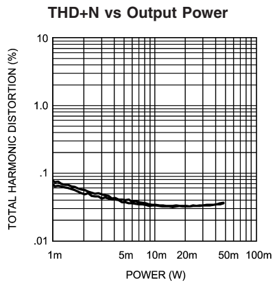
Analog V_{DD} = 5V , Digital V_{DD} = 3V R_L = 32\Omega , 44.1 kHz Sample Rate R & L Channels, Vol = 3dB, Frequency in = 1kHz
