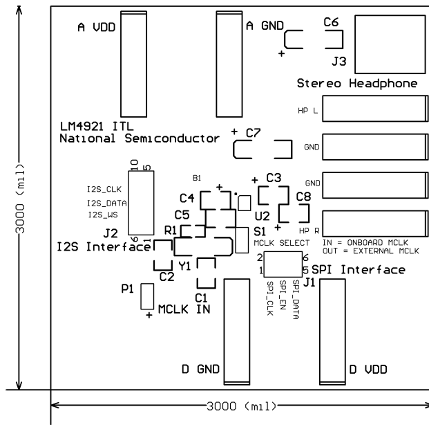
Silkscreen Layer
