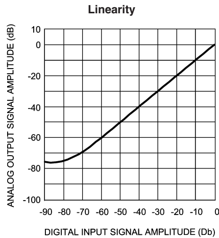
200486E2 Analog V_{DD} = 3V , Digital V_{DD} = 3V R_L = 32\Omega , 44.1kHz Sample Rate
