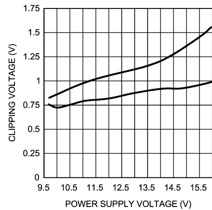
R_L = 4\Omega , f_{IN} = 1\text{kHz} at (from top to bottom at 12.5\text{V} ): positive signal swing, negative signal swing
