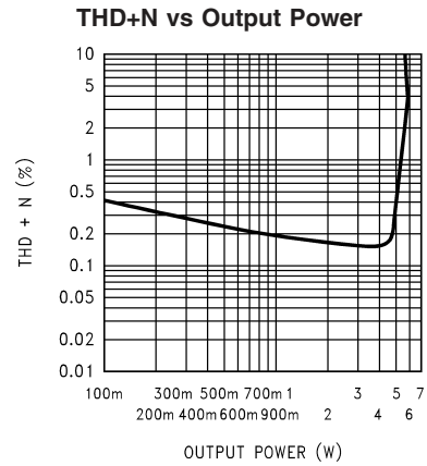
V_{DD} = 16\text{V} , R_L = 4\Omega , f_{IN} = 1\text{kHz}
