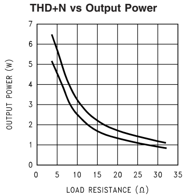
V_{DD} = 15\text{V} , at (from top to bottom at 15\Omega ): \text{THD+N} = 10\% , \text{THD+N} = 1\% , f_{IN} = 1\text{kHz}
