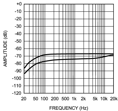
V_{DD} = 16\text{V} , R_L = 4\Omega , P_{OUT} = 1\text{W} , Input Referred at (from top to bottom at 1\text{kHz} ): V_{INB} driven, V_{OUTA} measured; V_{INA} driven, V_{OUTB} measured
