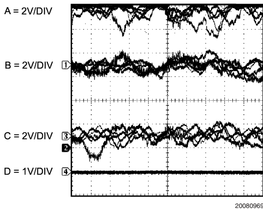
FIGURE 8. Same conditions and waveforms as shown in Figure 7, except that a 10\mu\text{F} capacitor has been connected between the DC VOL pin and GND (Trace C)
