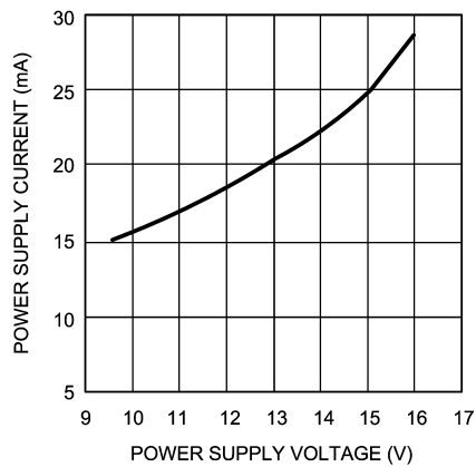
R_L = 4\Omega , V_{IN} = 0\text{V} , R_{SOURCE} = 50\Omega
