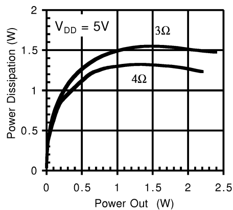
LM4867LQ, LM4867MTE Power Dissipation vs Power Output
