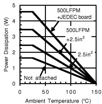
LM4867MTE (Note 18) Power Derating Curve
