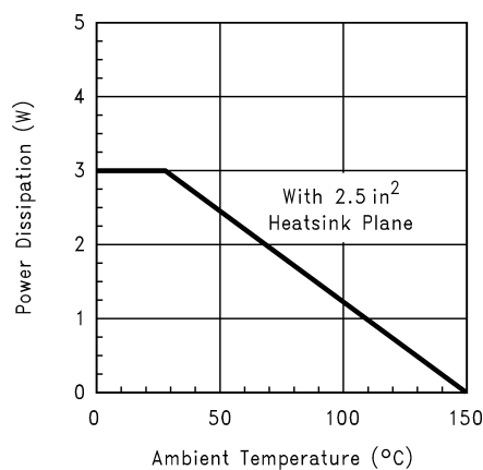
LM4867LQ Power Derating Curve
