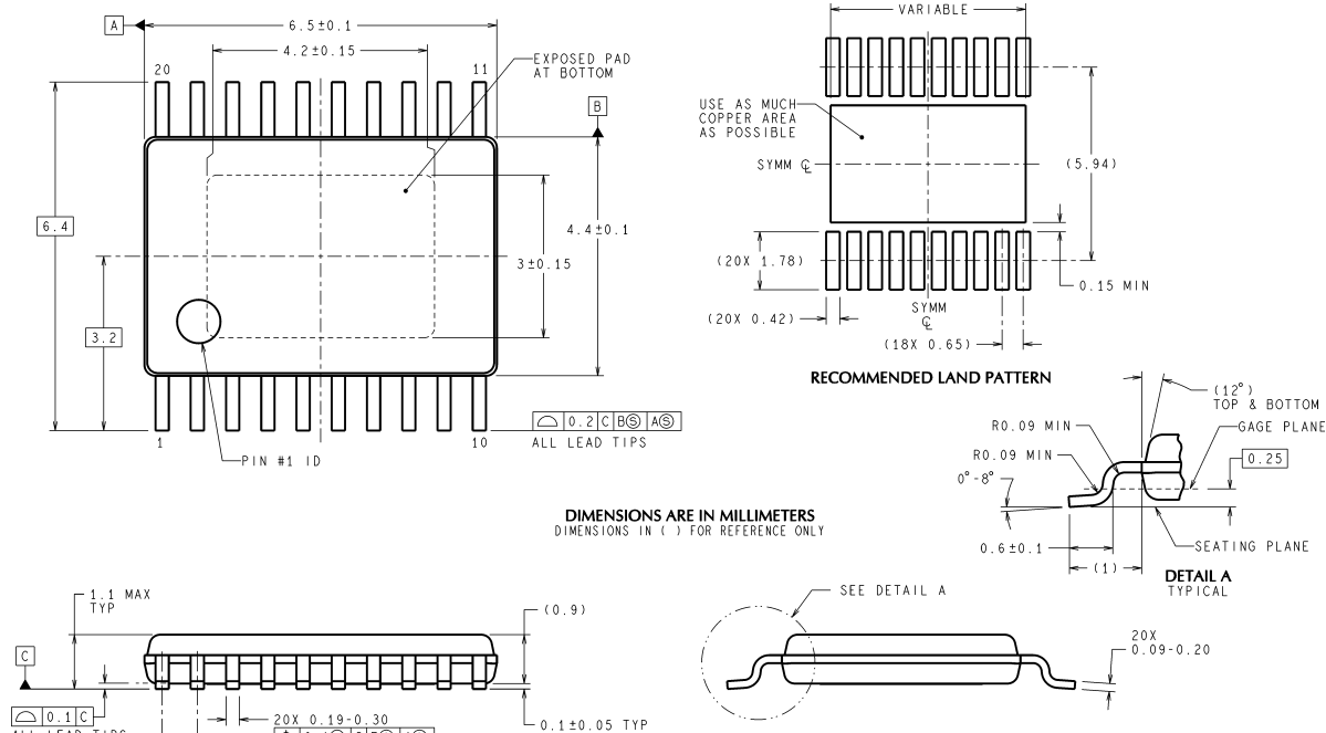
20-Lead MOLDED TSSOP, EXPOSED PAD, 6.5x4.4x0.9mm Order Number LM4867MTE NS Package Number MXA20A
