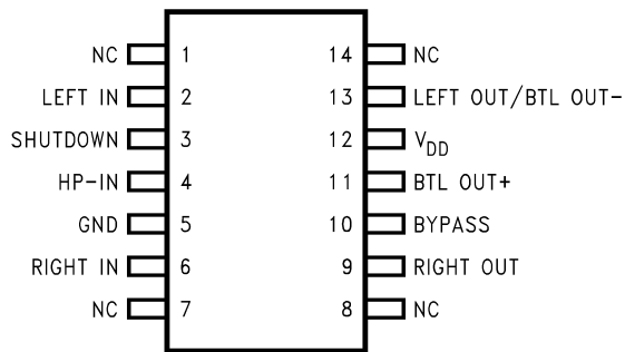
Top View 14 Lead TSSOP Order Number LM4850MT See NS Package Number MTC14
