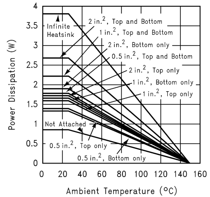
LM4850LD (Note 13) Power Derating Curve
