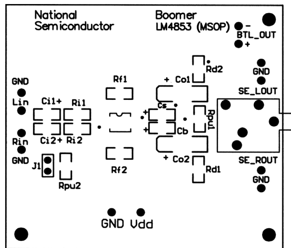
FIGURE 3. Recommended MM PCB Board Layout: Component-Side SilkScreen
