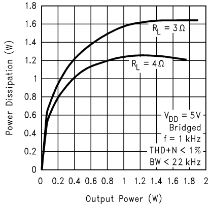
LM4853LD Power Dissipation vs Output Power
