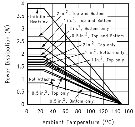
LM4853LD Power Derating Curve
