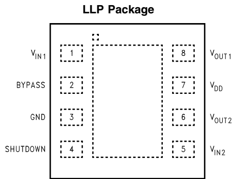
Top View Order Number LM4810LD See NS Package Number LDA08B
