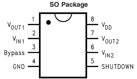
Top View Order Number LM4810MA See NS Package Number M08A
