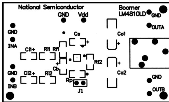
FIGURE 6. Recommended LD PC Board Layout Component-Side Silkcreen
