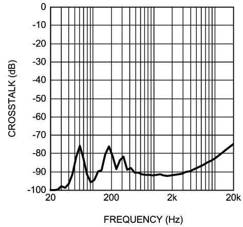
Crosstalk vs Frequency V_{DD} = 3.3V , R_L = 32\Omega , P_O = 12mW Right-Left, OCL, Mode 4
