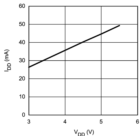
Supply Current vs Supply Voltage R_L = 32\Omega , SE, Mode 4
