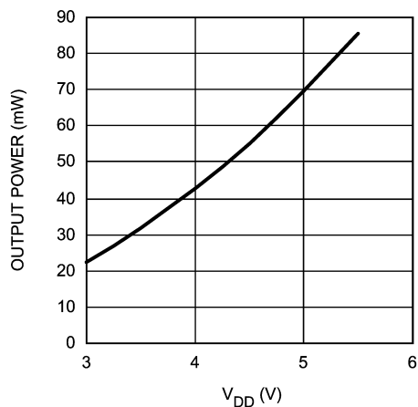
Output Power vs Supply Voltage R_L = 32\Omega , SE, Mode 6
