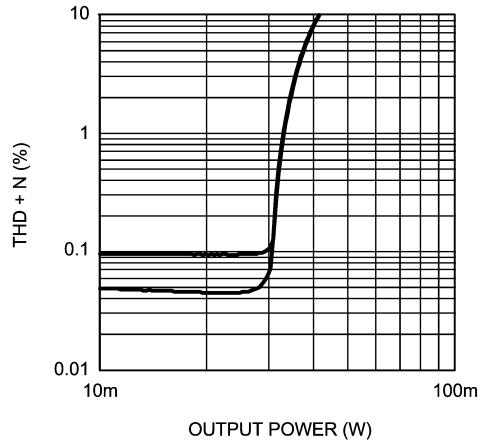
THD+N vs Output Power V_{DD} = 3.3V , R_L = 32\Omega , f = 1kHz Mode 6, OCL
