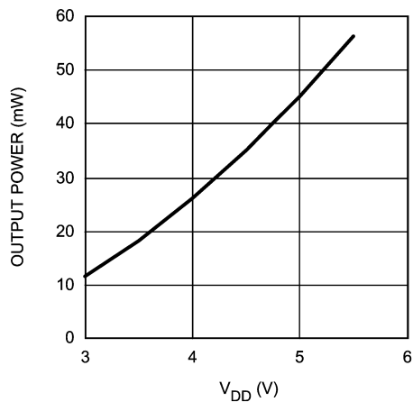
Output Power vs Supply Voltage R_L = 32\Omega , OCL, Mode 6
