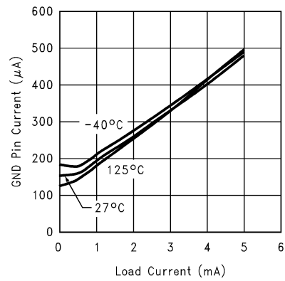
GND Pin Current vs Load
