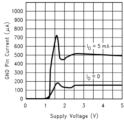
GND Pin Current
