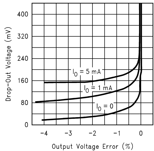
Dropout Voltage vs Output Error
