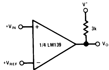
Basic Comparator
