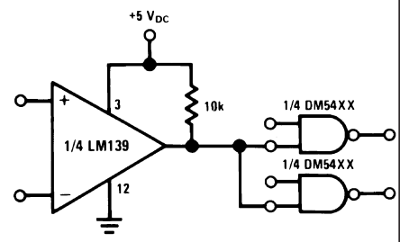
Driving TTL
