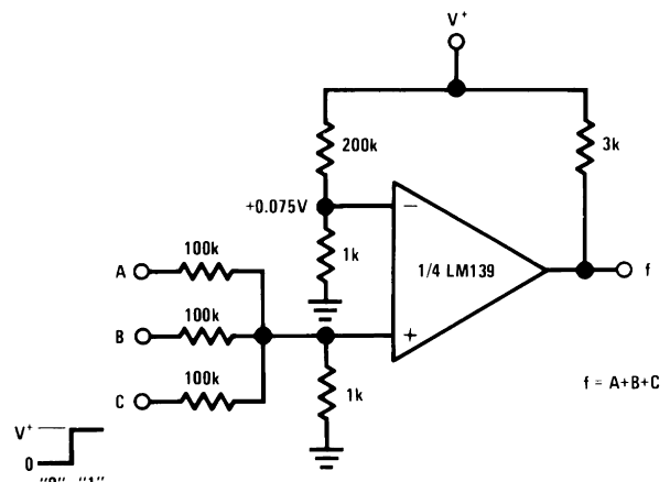
OR Gate
