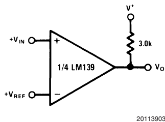
Basic Comparator
