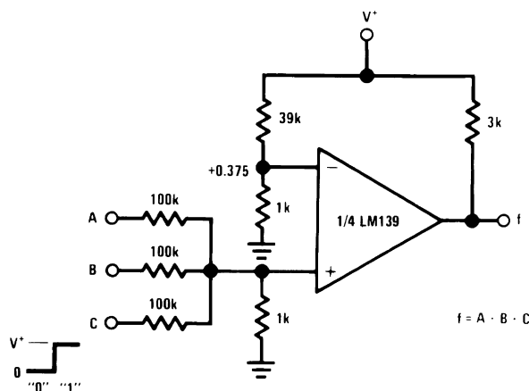
AND Gate
